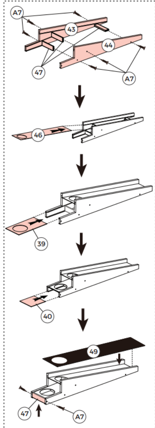
FIG. 10B Assembly
